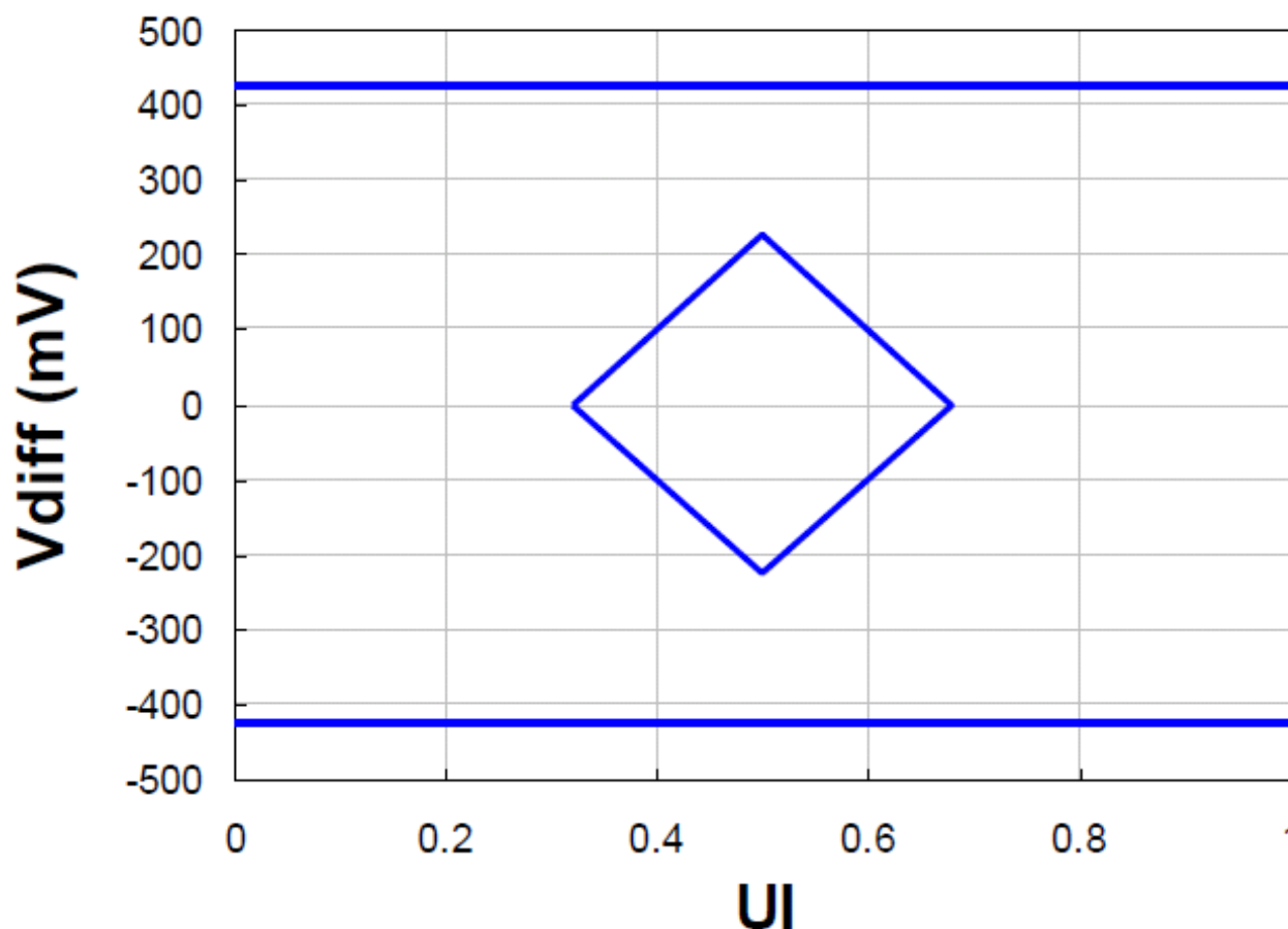
Figure 2 – QSFP+ Receiver Output Differential Signal Mask
