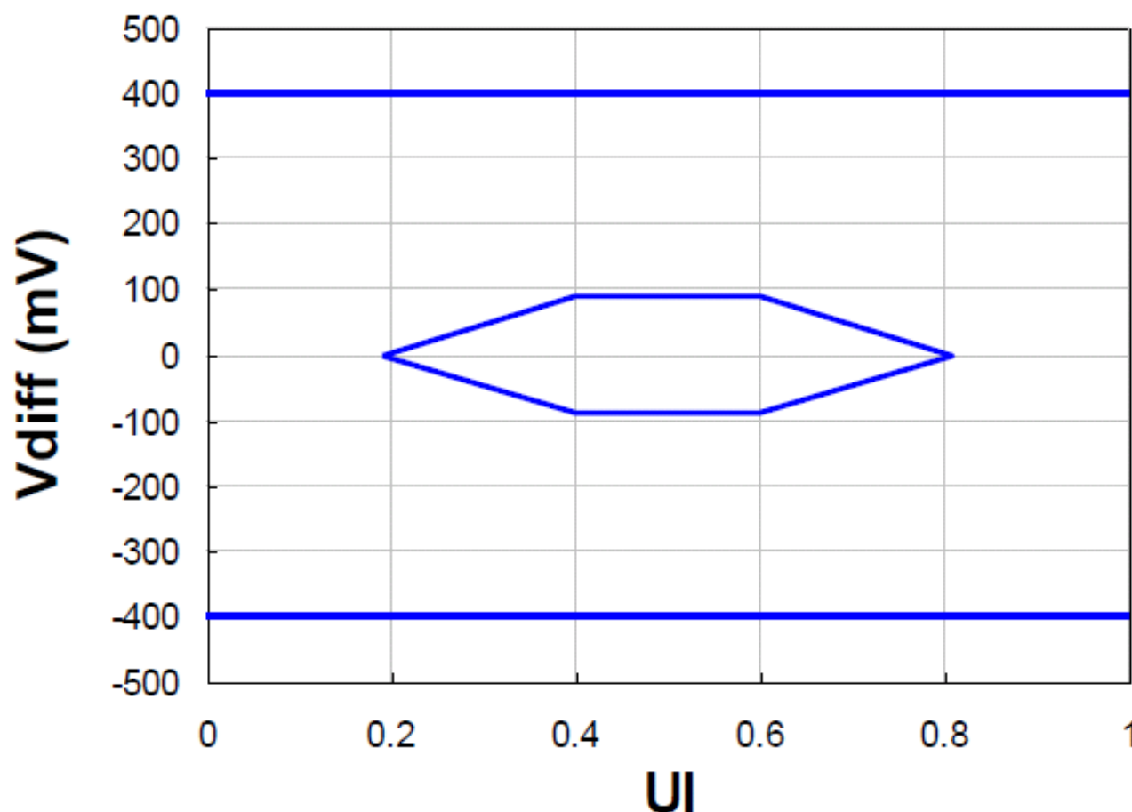
Figure 1 – QSFP+ Transmitter Input Differential Signal Mask
